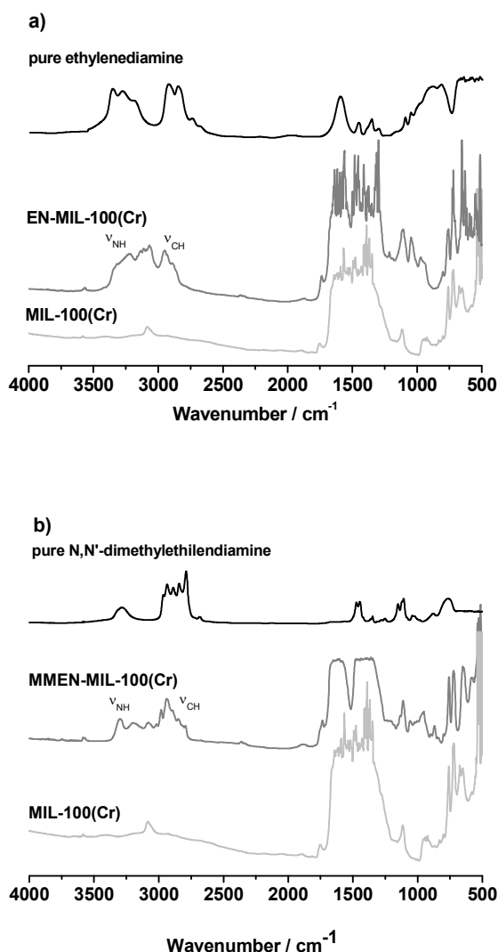
Fig. 3 FTIR spectra of the bare MIL-100(Cr) and the functionalized samples: EN-MIL-100(Cr) (a) and MMEN-MIL-100(Cr) (b) degassed at 423 K. Pure amines (in liquid phase) spectra are shown for comparison.
