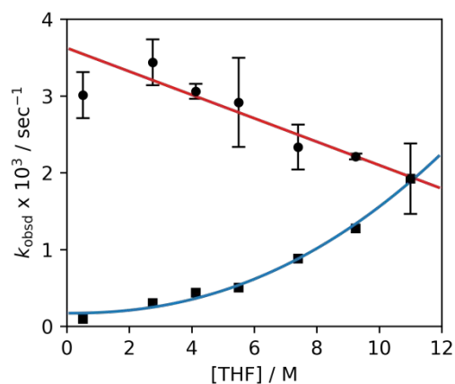
Figure 5. Plot of k_{\text{obsd}} versus THF concentration for alkylation of 0.025 M 4g with allyl bromide (0.275 M) in 0.250 M free HMPA 21 at -78 °C in toluene (■) or 2,5-Me 2 THF (●) co-solvent. The blue curve depicts an error-weighted least-squares fit to f(x) = y_0 + ax^b such that y_0 = 1.71 \times 10^{-4} \pm 0.57 \times 10^{-4} , a = 8.16 \times 10^{-6} \pm 5.10 \times 10^{-6} , b = 2.2 \pm 0.2 . The red curve depicts an error-weighted least-squares fit to f(x) = y_0 + ax such that y_0 = 3.62 \times 10^{-3} \pm 0.14 \times 10^{-3} , a = -1.5 \times 10^{-4} \pm 0.17 \times 10^{-4} .
