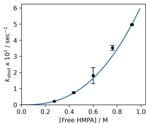
Figure 4. Plot of k_{\text{obsd}} against [\text{HMPA}]_{\text{free}} for the alkylation of enolate 4g (0.025 M) with 0.275 M allyl bromide in 9.24 M THF/2,5-Me 2 THF at -78 °C. 21 The blue curve depicts an error-weighted least-squares fit to f(x) = ax^b such that a = 0.061 \pm 0.001 , b = 2.56 \pm 0.01 .
