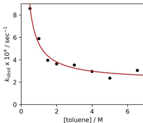
Figure 6. Plot of k_{\text{obsd}} versus toluene concentration for the alkylation of 0.025 M 4g at -78 °C with 0.275 M allyl bromide in 0.250 M free HMPA in 0.275 M THF using cyclopentane cosolvent. 21 The curve depicts a least-squares fit to f(x) = y_0 + ax^b such that y_0 = 2.13 \times 10^{-4} \pm 0.58 \times 10^{-4} , a = 3.30 \times 10^{-4} \pm 0.79 \times 10^{-4} , b = -0.98 \pm 0.24 .
