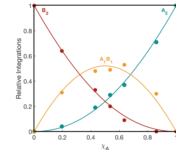
Figure 2. Job plot showing relative integrations of homodimers of 4g ( A_2 , blue) and 4i ( B_2 , red) and the heterodimer ( A_1B_1 , orange) plotted against the measured mole fraction 15 of 4g ( \chi_A ) for 0.20 M mixtures of sodium enolates 4g and 4i in 0.88 M TMEDA/toluene at -80^\circ\text{C} monitored by ^{13}\text{C}\{^1\text{H}\} NMR spectroscopy. The curves result from a parametric fit to a dimer model.
