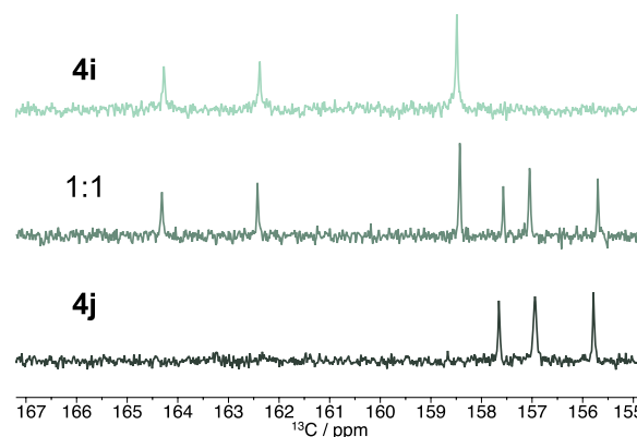
Figure 1. Partial 13 C NMR spectra of 0.20 M of 4i , a 1:1 mixture of enolates 4i and 4j , and 4j in THF at –20 °C. No new peaks appear indicating the absence of heteroaggregation consistent with a monomeric enolate.
