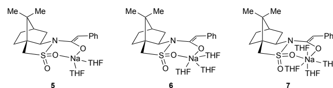
Scheme 1. The N -acyl camphorsultam derivatives and their enolates that are studied in this work.
