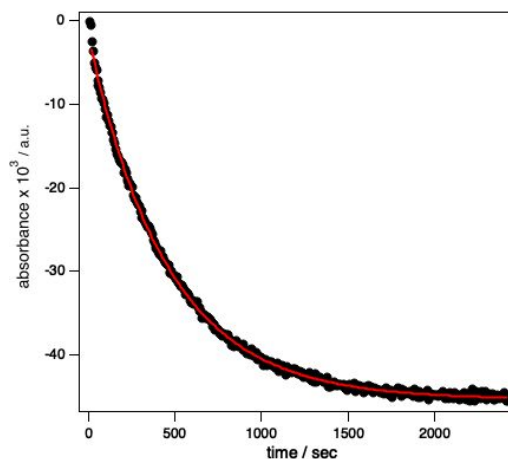
Figure 3. Alkylation of 4g (0.025 M; 1616 cm -1 ) with 0.275 M allyl bromide in 9.24 M THF/toluene at -78 °C to form 14 (1701 cm -1 ). The red curve depicts an unweighted least-squares fit to eq 4, such that n = 1.00 \pm 0.01 , k_{\text{obsd}} = 0.0022 \pm 0.0009 , and [\text{enolate}]_0 = 0.0430 \pm 0.0001 .
