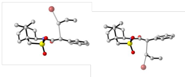
Figure 7. DFT computed transition structure for the alkylation of enolate 4g with allylbromide. Si -facial approach of the electrophile is favored (2.6 kcal mol -1 ) over the re face due to stereoelectronic effects emanating from the sultam sulfonyl moiety. 4
