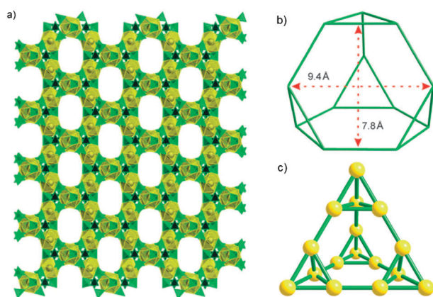
Fig. 1 (a) A view along [110] of the 3D structure of NDTB-1 . The disordered \text{H}_2\text{BO}_3^- anions and water residing in the channels have been omitted for clarity. (b) Cage topology of the structure of NDTB-1 . (c) Topology of the supertetrahedral 3D framework based on Th atoms (yellow).
