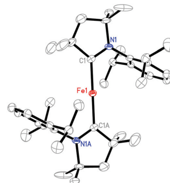
Fig. 2 Molecular structure of the cation [(Me 2 -cAAC) 2 Fe] + in 4 showing one of the two crystallographically independent cations in the unit cell with 30% probability ellipsoids.
