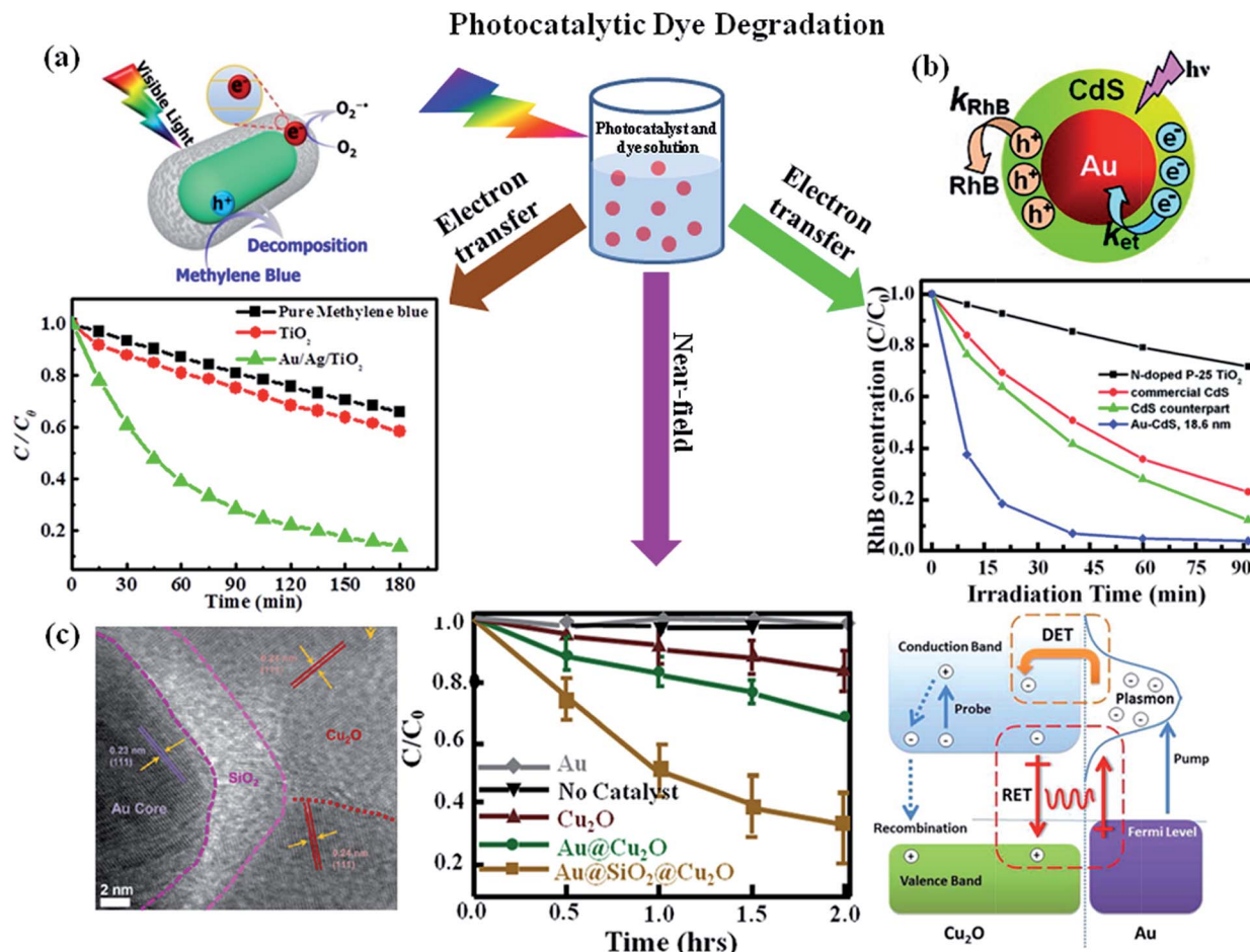
Fig. 9 Photocatalytic dye degradation: (a) photocatalytic degradation of MB under visible light irradiation in the absence and presence of photocatalysts ( \text{P25-TiO}_2 , \text{Au}/\text{TiO}_2 or \text{Au}/\text{Ag}/\text{TiO}_2 core-shell NPs) and the schematic representation for the mechanism of photocatalytic degradation of dyes upon visible light excitation of \text{Au}/\text{TiO}_2 NRs. (b) Photocatalytic degradation of RhB in the presence of \text{Au}/\text{CdS} , \text{CdS} and \text{P25-TiO}_2 . The data shows that \text{Au}/\text{CdS} NPs exhibit higher catalytic activity and the proposed mechanism to explain the plasmonic metal enhancement is shown in schematic representation. (c) TEM image of \text{Au}/\text{SiO}_2/\text{Cu}_2\text{O} NP section, visible-light photodegradation of methyl orange versus time monitored without catalyst and with catalysts \text{Au} , \text{Cu}_2\text{O} control, \text{Au}/\text{Cu}_2\text{O} , and \text{Au}/\text{SiO}_2/\text{Cu}_2\text{O} nanostructures and the schematic representation of various transfer mechanisms for the enhanced catalytic activity of \text{Au}/\text{Cu}_2\text{O} nanostructure. Figures (a), (b) and (c) reproduced with permission from ref. 32, 92, and 57, respectively.
