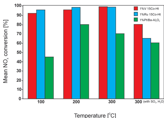
Fig. 6 Results of catalytic tests performed for Mg-Co-Al-O x . Reaction conditions: lean (120 s): 13.0% O 2 , 0.053% NO, 0.005% C 3 H 8 ; rich (60 s): 8.0% O 2 , 0.053% NO, 0.07% C 3 H 8 , N 2 balance; total flow rate = 650 ml min -1 ; mass of catalyst = 1000 mg (adapted from ref. 110 with kind permission from Elsevier).
