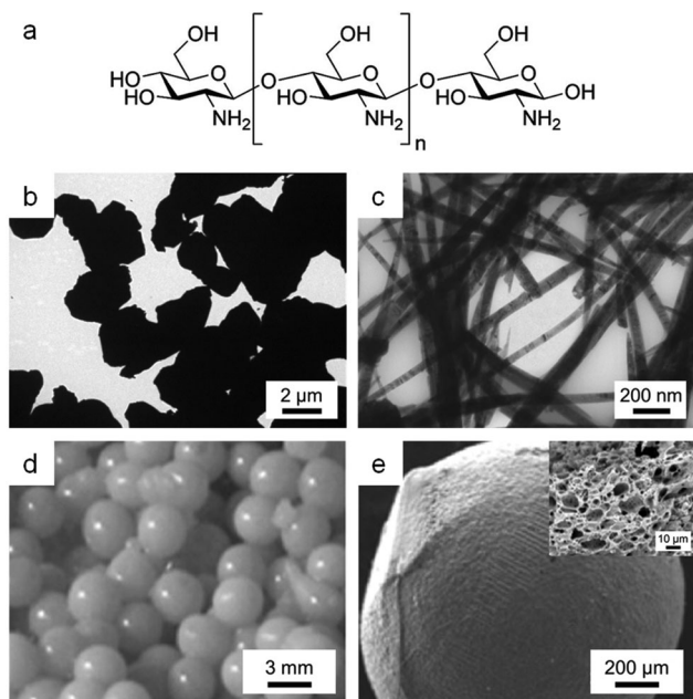
Fig. 12 (a) Structure of chitosan. TEM images of samples of \text{YBa}_2\text{Cu}_4\text{O}_8 synthesized using (b) acetate/tartrate and (c) chitosan. (d) Photograph and (e) SEM image of chitosan beads prepared by crosslinking with \text{Ce}^{3+} with (inset) SEM image of sponge-like structure formed after calcination of the beads. Images reproduced with permission from ref. 11 (b, c) and 109 (d, e).
