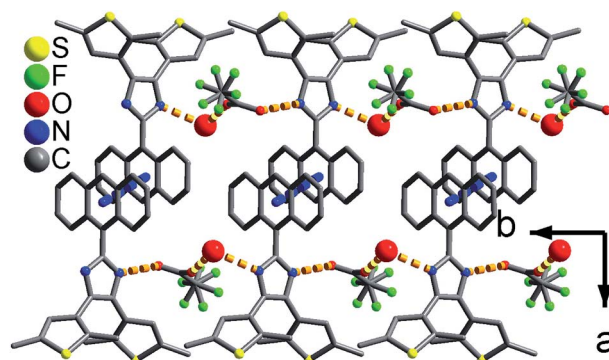
Fig. 4 The π...π stacking interactions between the anthracene moieties in 3. The red balls are the O atoms from the H 2 O molecules.
