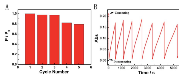
Fig. 4 (A) Repeated rechargeability test of the self-powered Mg/PB battery by simply disconnecting PB and Mg in 0.025 M NaClO, 1 M KCl and 0.1 M phosphate buffer (pH 6) electrolyte. (B) In situ absorbance measurement of the Mg/PB battery under repeated discharging and charging cycles.
