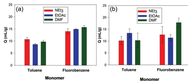
Fig. 2 Comparison of the swellability ( Q ) for toluene and fluorobenzene derived HCPs (prepared using 2 equivalents of FDA) against the three simulants triethylamine ( NEt_3 ), ethyl acetate (EtOAc), and dimethylformamide (DMF) using (a) Method 1 and (b) Method 2.
