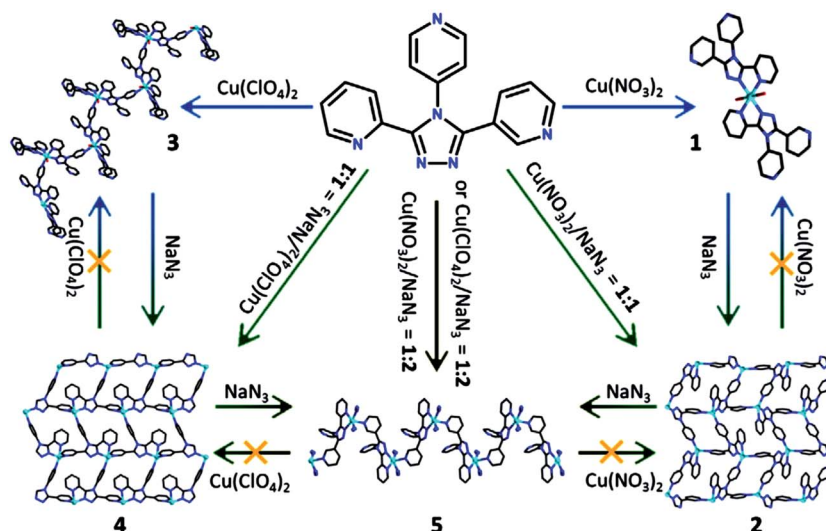
Scheme 12 A diagram illustrating self-assembled and structural transforming processes including 3-(2-pyridyl)-4-(4-pyridyl)1,2,4-triazole, metal salt Cu(NO 3 ) 2 or Cu(ClO 4 ) 2 , and NaN 3 . [Reprinted from ref. 138. Copyright 2015, with permission from Elsevier.]
