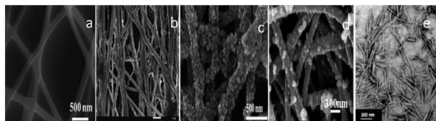
Fig. 1 SEM images of various types of CNF synthesized from cotton (a) natural electrospun CNF 56 (b) aligned CNF (scale bar 1 \mu m) 54 (c): CdS functionalized CNF 33 (d): CeO 2 functionalized CNF 56 (e): CNF prepared by acid hydrolysis 52 (adopted with permission).
