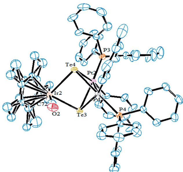
Fig. 16 Crystal structure of [\text{CpIr}(\text{CO})(\mu\text{-Te})_2(\text{PdTol}(\text{PPh}_3))] (redrawn from ref. 157).
