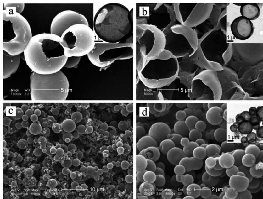
Fig. 7 SEM images of poly( o -toluidine) (POT) hollow microspheres synthesized at different [APS]/[ o -toluidine] ratios of: (a) 0.8 : 1 and (b) 0.6 : 1. (c) and (d) SEM images of POT hollow microspheres synthesized at different temperatures: (c) 25 °C and (d) −10 °C. The insets show the corresponding TEMs image of the POT hollow structures. Reproduced from ref. 76 with permission from John Wiley and Sons.
