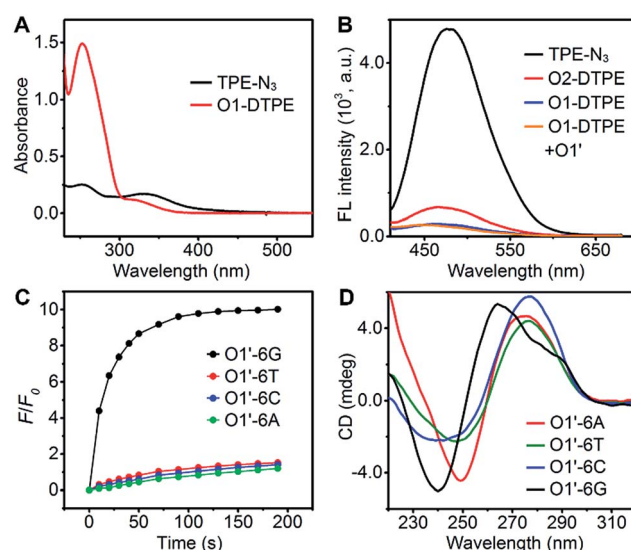
Fig. 2 (A) UV absorbance spectra of 10 μM TPE- \text{N}_3 and 10 μM O1-DTPE in DMSO/H 2 O (v/v, 1/399). (B) Fluorescence spectra of 1.0 μM TPE- \text{N}_3 , O2-DTPE, O1-DTPE, and the mixture of 1.0 μM O1-DTPE and O1' in TE reaction buffer at 25 °C. (C) F/F_0 of 1.0 μM O1-DTPE in the presence of 1.0 μM O1'-6G, O1'-6A, O1'-6C, and O1'-6T in TE reaction buffer at 25 °C. (D) CD spectra of 20 μM O1'-6G, O1'-6A, O1'-6C, and O1'-6T in TE reaction buffer at 25 °C.
