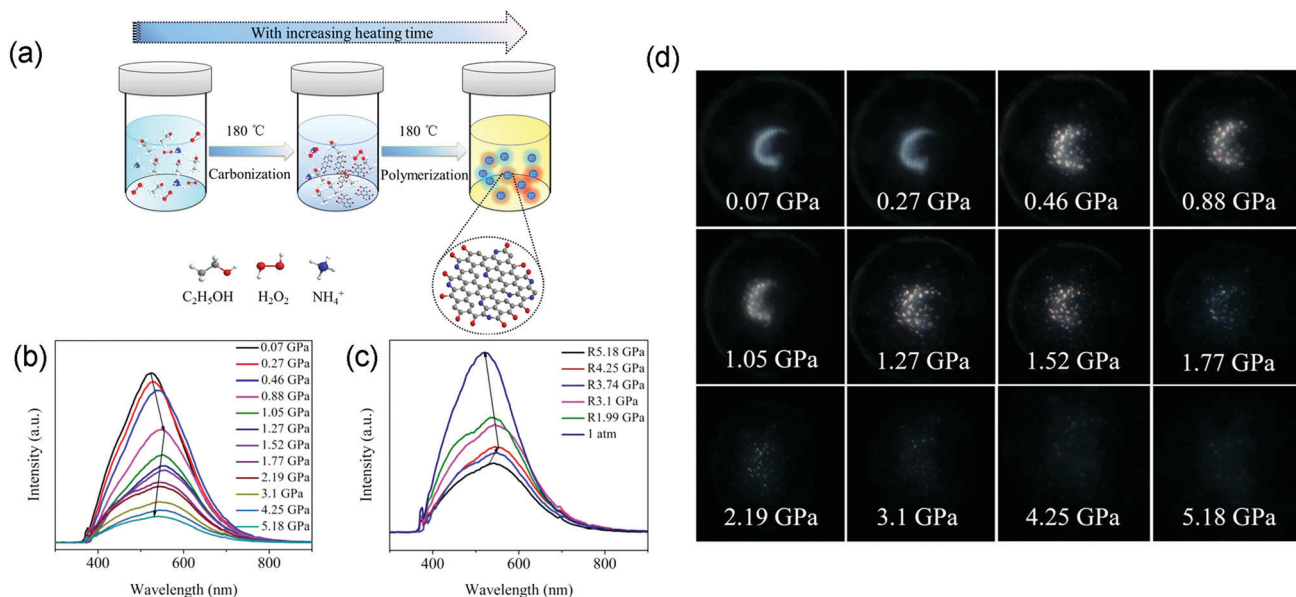
Fig. 5 (a) Schematic of the facile synthesis of N-CDs via a one-step ethanol-thermal strategy treated with H_2O_2 and NH_3 \cdot H_2O . (b) PL spectra of N-CDs with increasing pressure. (c) PL spectra of N-CDs as the pressure decreases to ambient conditions. (d) Optical photographs of N-CDs with increasing pressure. Reproduced with permission from ref. 43. Copyright 2018 American Chemical Society.
