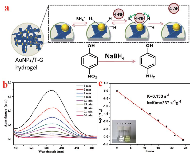
Fig. 8 Schematic of the Langmuir–Hinshelwood model for the catalytic reduction of 4-NP (a), UV-vis spectra for the catalytic reduction of 4-NP (b), plots of ln(C t /C 0 ) versus T for reduction process with the inserted photo of color change from 4-NP to 4-AP (c).
