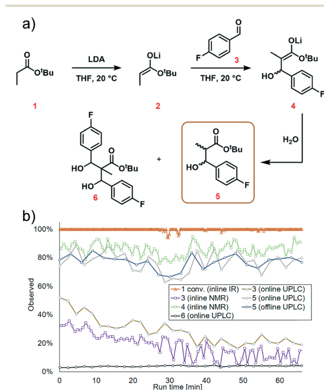
Fig. 7 Reaction data from the scale-out run. a) Overall reaction scheme, highlighting the species which were quantified; b) graph showing the quantity of each species over time, detected by different instruments.
