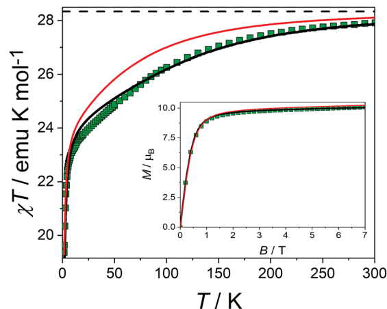
Fig. 3 Experimental (symbols), fitted (black line) and ab initio calculated product of the temperature times the magnetic susceptibility of a powder sample of Dy 2 , recorded with a static magnetic field B = 0.1 T. The dotted line represents the Curie constant for two independent Dy 3+ ions. Inset: magnetization recorded at T = 1.8 K with fields up to 7 T, same color code.
