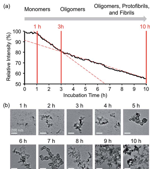
Fig. 3 Time-dependent fluorescent response and aggregation progression of Zn(II)-treated A-1 . (a) Change in the FRET signal of A-1 with Zn(II) as a function of incubation time. (b) TEM images of Zn(II)-added A-1 aggregates generated at various incubation time points (scale bar = 200 nm). Conditions: [ A-1 ] = 0.25 \mu M (for FRET) and 2.5 \mu M (for TEM); [ZnCl 2 ] = 100 \mu M (for FRET) and 1 mM (for TEM); \lambda_{\text{ex}} = 280 nm; \lambda_{\text{em}} = 420 nm; incubation up to 10 h; room temperature.
