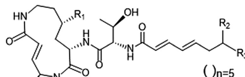
glidobactin A (9): R_1 = H , R_2 = H , R_3 = CH_3
