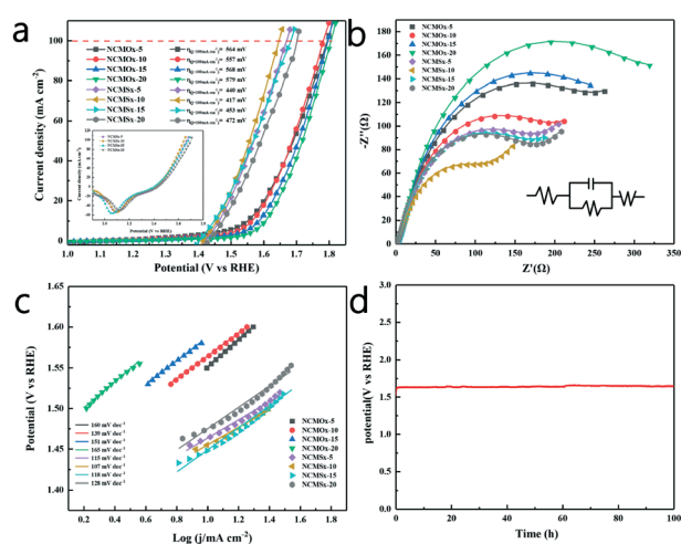
Fig. 6 (a) OER polarization curves (iR-corrected) at a scan rate of 2 mV s -1 ; (b) OER electrical impedance maps; (c) the Tafel slopes of the materials; and (d) results of the 100 h chronopotentiometry test of NCMS x-10 under the OER.
