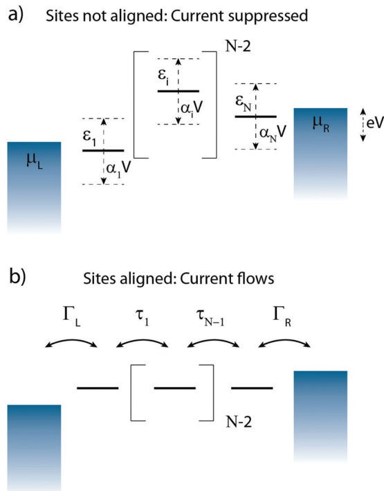
Fig. 2 N-Site model. Schematic representation of the N-site model, with the sites represented as short horizontal lines. (a) The sites, with on-site energy \varepsilon_i , are misalignment and the current is strongly suppressed. When a bias voltage V is applied across the molecule, each site experiences a shift of \alpha_i V . (b) If the sites are aligned, charge transport occurs efficiently. The outermost sites are coupled with \Gamma_{R,L} to their respective electrode, with the adjacent sites coupled by \tau_i .
