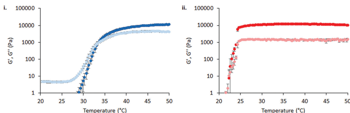
Fig. 5 Temperature ramp rheograms of 50% (w/v) PNIPAM 98 -PEG 122 -PNIPAM 98 (i) and 20% (w/v) poloxamer 407 (ii) in VFS at a fixed shear stress (1 Pa) and frequency (1 Hz). G' and G'' are shown as dark and light markers, respectively. Data presented as mean \pm standard deviation, n = 3 .
