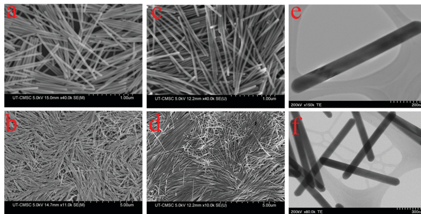
Fig. 1 SEM images of Te NWs obtained from \text{TeO}_2 with ethylene glycol at 120 °C (a) and (b) 0.1 g PVP and 0.75 mL ascorbic acid (c) and (d) 0.2 g PVP and 1.5 mL ascorbic acid and (e) and (f) STEM images of Te NWs obtained from 0.1 g PVP and 0.75 mL ascorbic acid.
