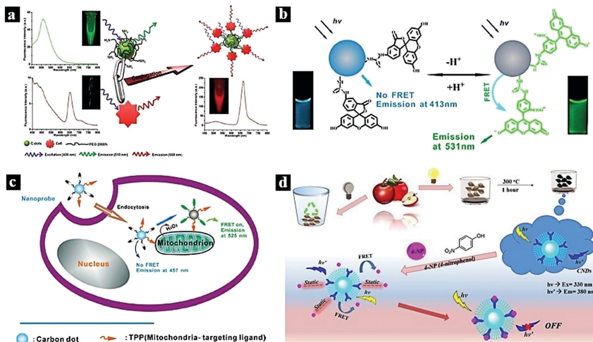
Fig. 2 (a) FRET process between CDots and chlorin e6. 8 Reprinted with permission ref. 8. Copyright 2012 Wiley. (b) Schematic illustration of a Cdot-based FRET nanoprobe for pH sensing. 33 Reprinted with permission ref. 33. Copyright 2013 IOP Publishing Ltd. (c) Nanoprobe using FRET-based H 2 O 2 ratiometric sensing in a living cell. 10 Reprinted with permission ref. 10. Copyright 2014 Wiley-VCH Verlag. (d) Schematic illustration of the synthetic process of CDots and the FRET process between CDots and 4-nitrophenol. 15 Reprinted with permission ref. 15. Copyright 2018 Elsevier.
