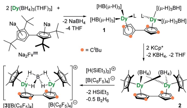
Scheme 1 Synthesis of compounds 1 , 2 and [\mathbf{3}][\text{B}(\text{C}_6\text{F}_5)_4] ( \text{L} = \text{THF} ).
