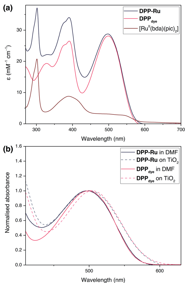
Fig. 2 (a) UV-vis absorption spectra of DPP dye , [\text{Ru}^{\text{II}}(\text{bda})(\text{pic})_2] and DPP-Ru in DMF solution. (b) Normalised UV-vis spectra of DPP dye and DPP-Ru on a mTiO 2 film coated on a glass slide, and in DMF solution.
