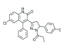
Fig. 5 Inhibitors of DSB repair by (A) NHEJ and (B) HR.
