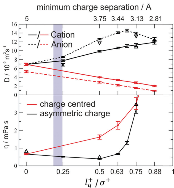
Fig. 16 Diffusion and viscosity as a function of charge separation. The blue shaded area indicates the l_q^+/\sigma^+ range for the [\text{C}_4\text{C}_{11}\text{im}] cation. The charge centred systems where charge separation is achieved by decreasing the size are shown in red. Reprinted (adapted) from H. V. Spohr and G. N. Patey, J. Chem. Phys. , 2009, 130 , 104506, with the permission of AIP Publishing. 217
