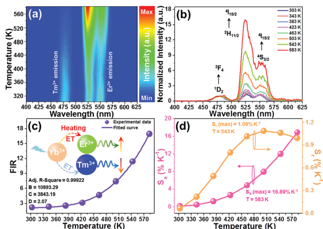
Fig. 5 (a) Contour lines of the Y 2 Mo 3 O 12 :Er 3+ /0.22Yb 3+ @BiOF:Tm 3+ /Yb 3+ (i.e., mass ratio = 1 : 5) composites as a function of temperature excited at 980 nm. (b) Temperature-dependent UC emission spectra (normalized at 480 nm) and (c) FIR value of the Y 2 Mo 3 O 12 :Er 3+ /0.22Yb 3+ @BiOF:Tm 3+ /Yb 3+ composites. (d) Dependence of the S a and S r values on the temperature.
