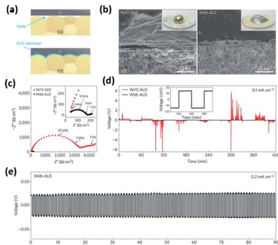
Fig. 7 Characterization of a garnet-type SSE/Li metal interface. (a) Schematic of the wetting behavior of the garnet surface with molten Li. (b) Scanning electron microscopy (SEM) images of the garnet-type SSE/Li metal interface. Without ALD- \text{Al}_2\text{O}_3 coating, the SSE has a poor interfacial contact with Li metal even on heating. With the help of ALD- \text{Al}_2\text{O}_3 coating on garnet, Li metal can uniformly bond with the SSE at the interface on heating. The inset shows the photos of melted Li metal on top of the garnet surface clearly demonstrating classical wetting behavior for the ALD-treated garnet-type SSE surface. (c) Comparison of Nyquist plots of the symmetric Li non-blocking garnet cells. The inset shows the enlarged impedance curve of the ALD-treated cell. (d) Comparison of dc cycling for symmetric cells at 0.1 \text{ mA cm}^{-2} . The inset shows the magnified curve of the ALD-treated cell. (e) Cell voltage profile during extended cycling. 27
