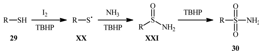
Scheme 15 Mechanism of reaction between thiols 29 and ammonia in the presence of I _2 and ^t\text{BuOOH} .
