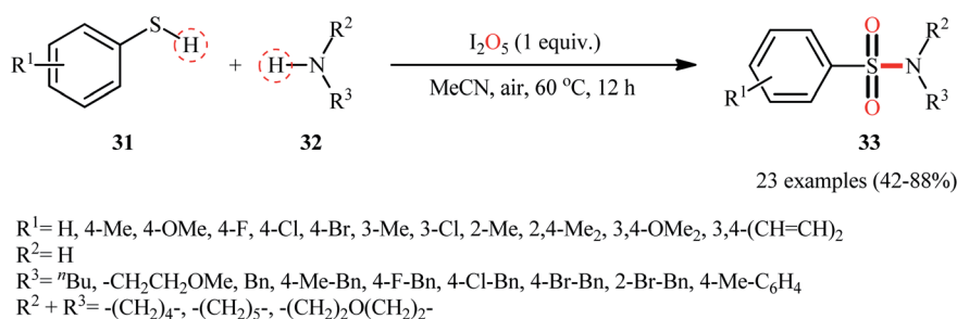
Scheme 16 Direct synthesis of sulfonamides 33 from thiols 31 and amines 32 through the action of I _2\text{O}_5 .
