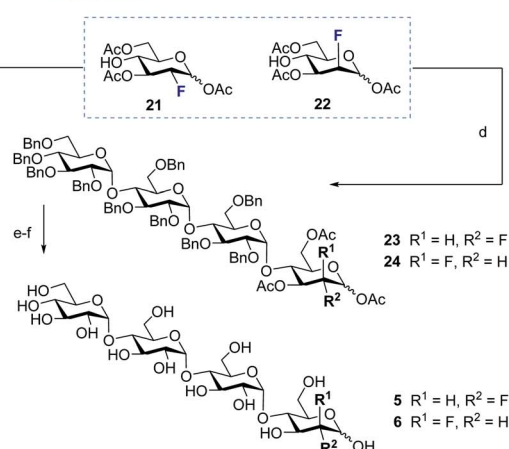
Scheme 2 Preparation of fluorinated maltotetraose cores 5 and 6 . Conditions: (a) Ac 2 O, DMAP, pyridine, 4 h, RT, 88%. (b) 4-Methylbenzenethiol, BF 3 ·OEt 2 , CH 2 Cl 2 , 23 h, RT, 78%. (c) (1) NaOMe, MeOH, 2 h, RT, 91%; (2) NaH, BnBr, TBAL, DMF, 20 h, RT, 77%. (d) NIS, BF 3 ·OEt 2 , CH 2 Cl 2 , 15 min, RT, 23 : 21%, 24 : 25%. (e) Pd/C, H 2 , MeOH, EtOAc, 24 h, RT; (f) NaOMe, MeOH, 8 h, RT, 5 : 88%, 6 : 67% over two steps.
