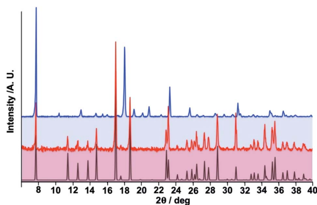
Fig. 6 Comparison of calculated and experimental (black and red lines) powder X-ray diffraction (PXRD) patterns for 1 \cdot \text{PhNO}_2 with the experimental PXRD of 1 (blue line).
