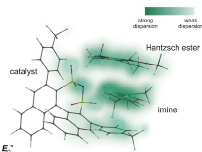
Fig. 4 (A) E_O'' and E_{N,I}'' shown here are the computed lowest-energy conformations of the ternary complex \text{CF}_3\text{-DSI } 2b/E\text{-}5b/3c . E_O'' accommodates all the experimental NOE and HOESY connections (key NOEs/HOEs are shown in the structures computed at TPSS-D3(BJ)/def2-SVP/SMD). Table 1 shows \Delta G_{(\text{DCM},180\text{ K})} for the principal conformations (free energy corrections and solvation corrections at the geometry optimization level of theory were added to the single-point total electronic energies). Table 2 illustrates the relative stabilities \Delta G_{(\text{DCM},180\text{ K})} of the conformationally refined structures. (B) Binding of the Hantzsch ester occurs at the oxygen atoms as evidenced by electrostatic potential map of the binary E_N and ternary E_O complexes. (C) Noncovalent interaction plot of complex E_O'' , suggesting that dispersion contributes significantly to stabilization of the ternary complex. (D) Dispersion interaction density plot confirms the importance of dispersion within complex E_O'' (computed at DLPNO-CCSD(T)/def2-TZVP level of theory).
