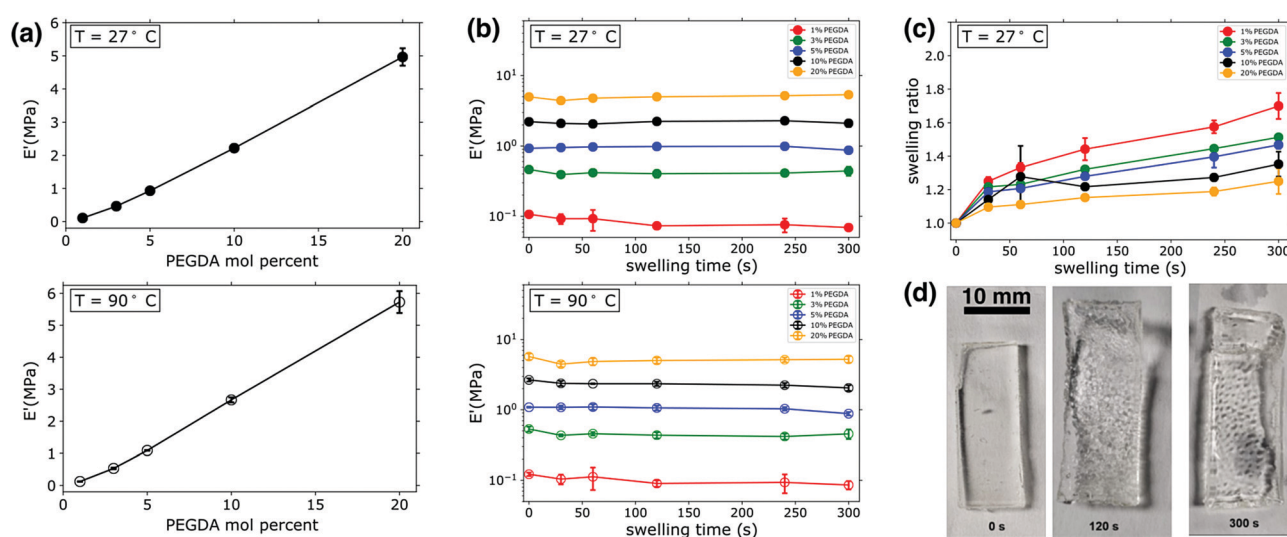
Fig. 1 (a) Gel storage modulus vs. PEGDA mol percent at T = 27^\circ\text{C} (upper panel) and T = 90^\circ\text{C} (lower panel). (b) Gel storage modulus as a function of swelling time at T = 27^\circ\text{C} (upper panel) and T = 90^\circ\text{C} (lower panel). (c) Swelling ratio at T = 27^\circ\text{C} . (d) Images of a PEG-hydrogel (3 : 97 PEGDA : PEGMEA) during the swelling process; the last panel shows the ruptured gel. This rupturing occurred in samples having 3–20 mol percent PEGDA, with rupturing occurring in roughly 10–20% of specimens.
