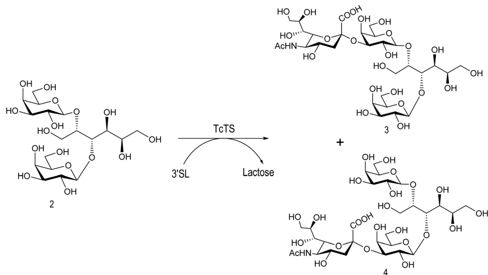
Scheme 6 Sialylation of 2,3-di-O-( \beta -D-Galp)- \beta -D-Galp alditol by TcTS. Adapted from ref. 130.
