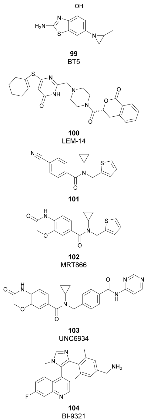
Fig. 28 NSD1–3 inhibitors.
