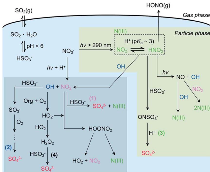
Fig. 2 Proposed multiphase oxidation of SO 2 promoted by particulate nitrate photolysis. Reprinted with permission from ref. 11 Copyright 2019 American Chemical Society.
