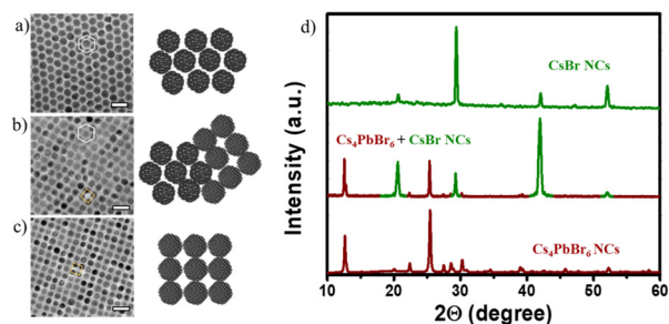
Fig. 5 (a–c) TEM images of NCs with two different packings (hexagonal close packing, HCP, and cubic close packing, CCP) while the reaction condition was transferring from \delta_2 to \delta_3 . Scale bars are 20 nm in all the images. (d) Powder XRD patterns of the samples in the regions of \delta_2 and \delta_3 corresponding to \text{Cs}_4\text{PbBr}_6 and \text{CsBr} NCs along with their mixed region.
