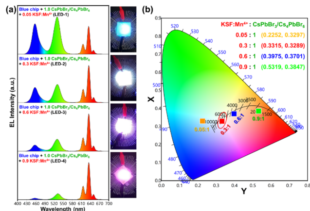
Fig. 9 (a) The electroluminescence spectra of the designed LED devices by varying the K 2 SiF 6 :Mn 4+ to CsPbBr 3 /Cs 4 PbBr 6 ratio in the wt% of 0.05:1, 0.3:1, 0.6:1, and 0.9:1 under forward-bias current of 20 mA (inset images are photographs of the working LEDs (LED 1–4)), (b) the CIE chromaticity coordinates corresponding to the constructed LED devices using different composite wt% ratios.
