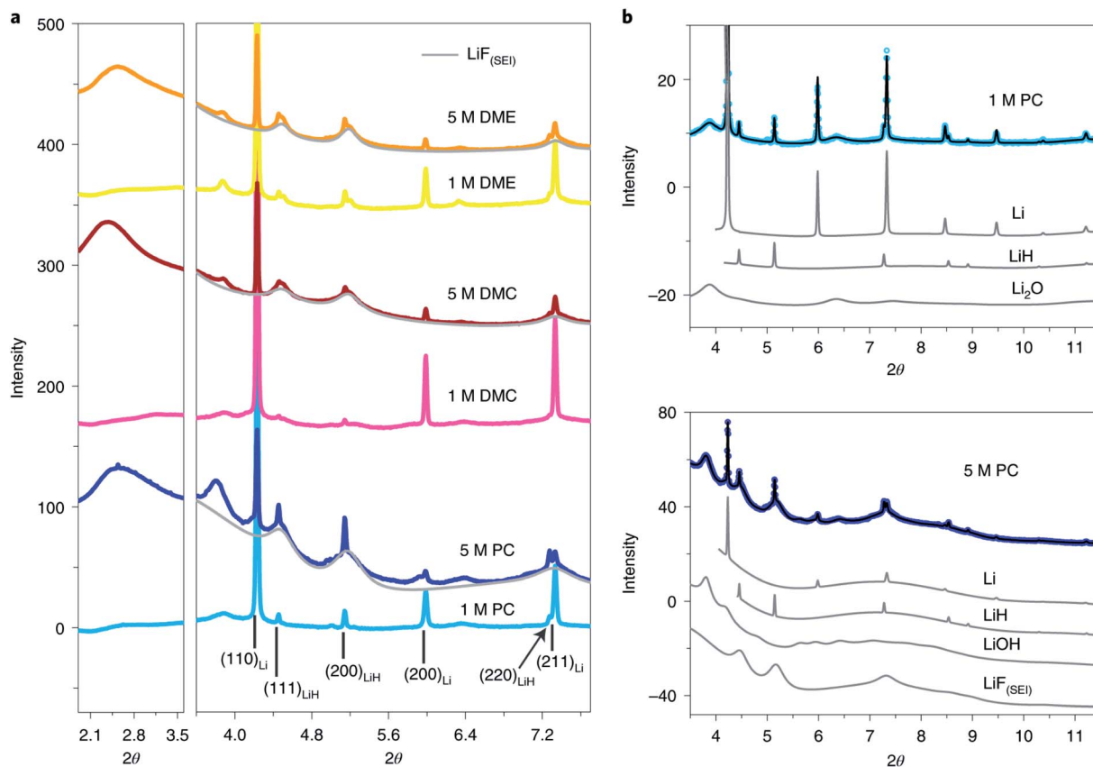
Fig. 9 (a) SEI XRD of LCEs and HCEs using LiFSI as the salt and PC, DMC and DME as the solvents. The light grey pattern belongs to LiF (SEI) . The wavelength used is 0.18323 Å. (b) Rietveld refinement of SEI XRD data of low- (upper) and high-concentration (lower) LiFSI in PC. Contributions of individual phases to the XRD pattern are also shown. Open circles, experimental data; black lines, calculated data. Reproduced with permission. 84 Copyright © 2021, Springer Nature Limited.
