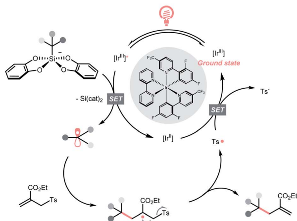
Scheme 51 Silicate-based reagents as R • precursors.
