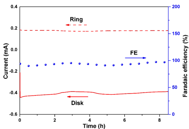
Fig. 7 Chronoamperometry stability test of CA-NR on RRDE at 1600 rpm ( 0.65 \text{ V vs. RHE} in 0.1 \text{ M KOH} ).
