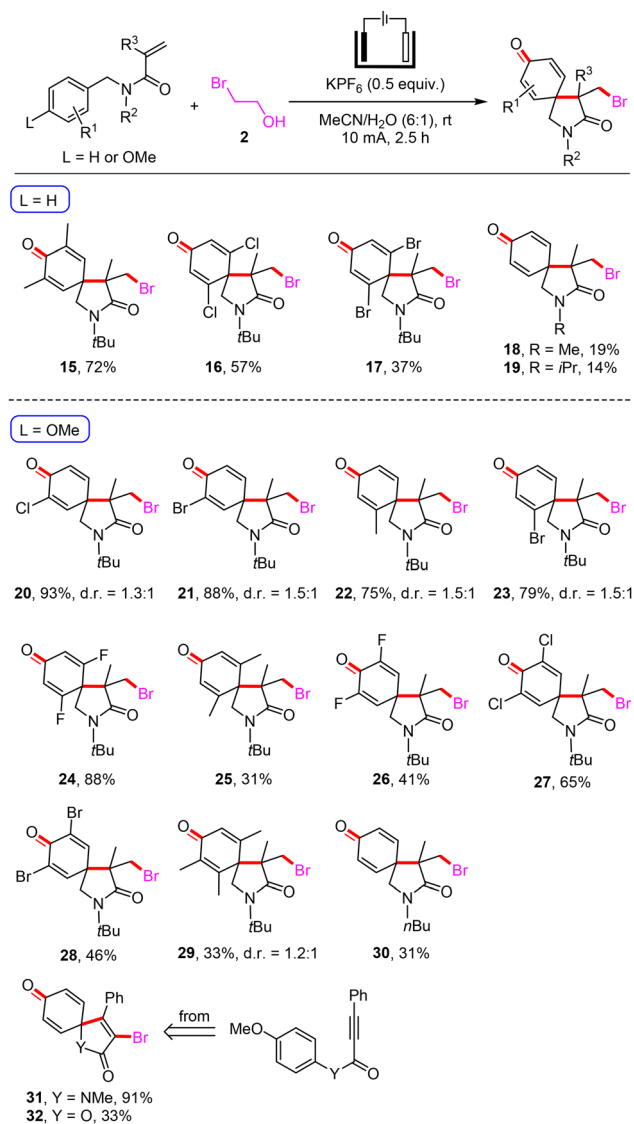
Scheme 3 Scope of the electrochemical bromination/spirocyclization [Reaction conditions: RVC anode, Pt cathode, undivided cell, acrylamide (0.20 mmol), 2-bromoethan-1-ol ( 2 , 0.60 mmol), KPF 6 (0.10 mmol), MeCN/H 2 O (6.0 mL/1.0 mL), rt, 10 mA, 2.5 h (4.6 F mol -1 ); isolated yields; d.r. = diastereomeric ratio].
