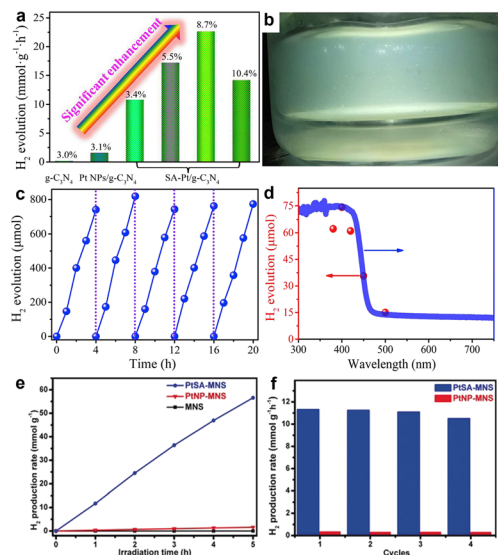
Fig. 4 (a) Visible light ( \lambda > 420 nm) photocatalytic HER activity of g-C 3 N 4 , Pt NPs/g-C 3 N 4 -K and SA Pt/g-C 3 N 4 -8.7; (b) Photos of reaction using 10 mg SA Pt/g-C 3 N 4 -8.7; (c) Stability test and (d) SA Pt/g-C 3 N 4 -8.7 of the apparent quantum test. Reprinted with permission from ref. 33. Copyright 2020, Elsevier; (e and f) Characterization of photocatalytic activity, (e) photocatalytic production rates of H 2 of Pt SA MNS, Pt NP MNS and MNS and (f) cyclic stability of Pt SA MNS and Pt NP MNS. Reprinted with permission from ref. 34. Copyright 2019, Wiley-VCH GmbH.
