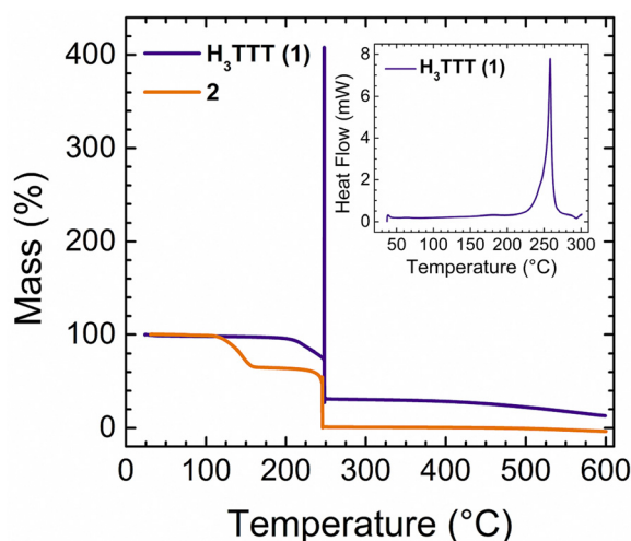
Fig. 3 Thermogravimetric analysis (TGA) of compounds 1 and 2, performed using a temperature ramp of 10 °C \text{min}^{-1} . The significant increase in mass percent observed at 247 °C in 1 is associated with the detonation of the material. (inset) Differential scanning calorimetry (DSC) of 1, also performed at 10 °C \text{min}^{-1} .
