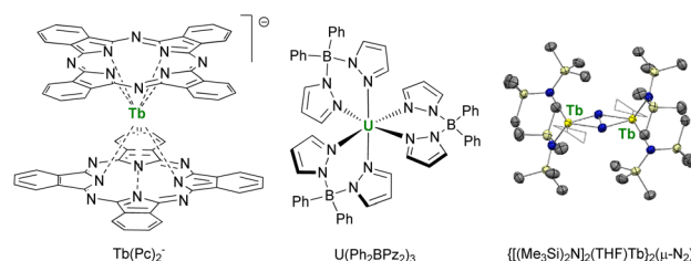
Fig. 6 Molecular structures of \text{Tb}(\text{Pc})_2 , 70 \text{U}(\text{Ph}_2\text{BPz})_3 , 176,177 and ORTEP plot of \{[(\text{Me}_3\text{Si})_2\text{N}]_2(\text{THF})\text{Tb}_2(\mu\text{-N}_2)^-\} , 180 (terbium atoms are in yellow, nitrogen atoms in blue, silicon atoms in pale yellow, carbon atoms in grey, hydrogen atoms are not represented, and coordinated thf molecules are represented in wireframe).
