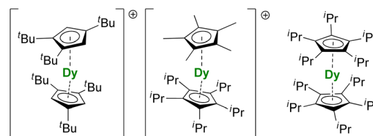
Fig. 8 Molecular structures [Dy(Cp^{ttt})_2]^+ , 72,73 [Dy(Cp^*)_2(μ-bipym)]^+ , 74 and Dy(Cp^{iPr5})_2 . 193
