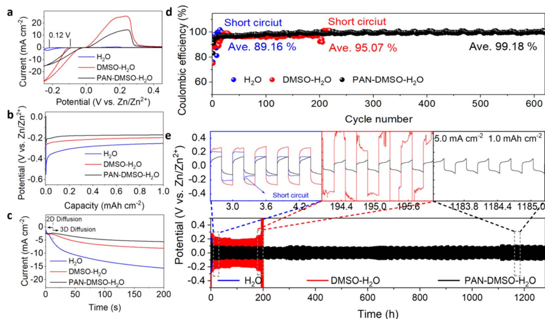
Fig. 3 (a) Cyclic voltammetry curves for Zn plating/stripping in different electrolytes at a scan rate of 1.0 mV s -1 . (b) Nucleation overpotential for Zn-Zn symmetric batteries and (c) potentiostatic current-time transient curves of the Zn electrodes in different electrolytes measured at -150 mV. (d) coulombic efficiency of Zn-Ti batteries in different electrolytes. (e) Cycling performance of Zn-Zn symmetric batteries containing different electrolytes at a current density of 5.0 mA cm -2 and an areal capacity of 1.0 mA h cm -2 . The blue, red and black lines represent the pristine aqueous, DMSO-H 2 O and PAN-DMSO-H 2 O electrolytes, respectively.
